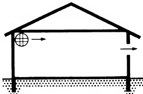
4 Pressurised ventilation
